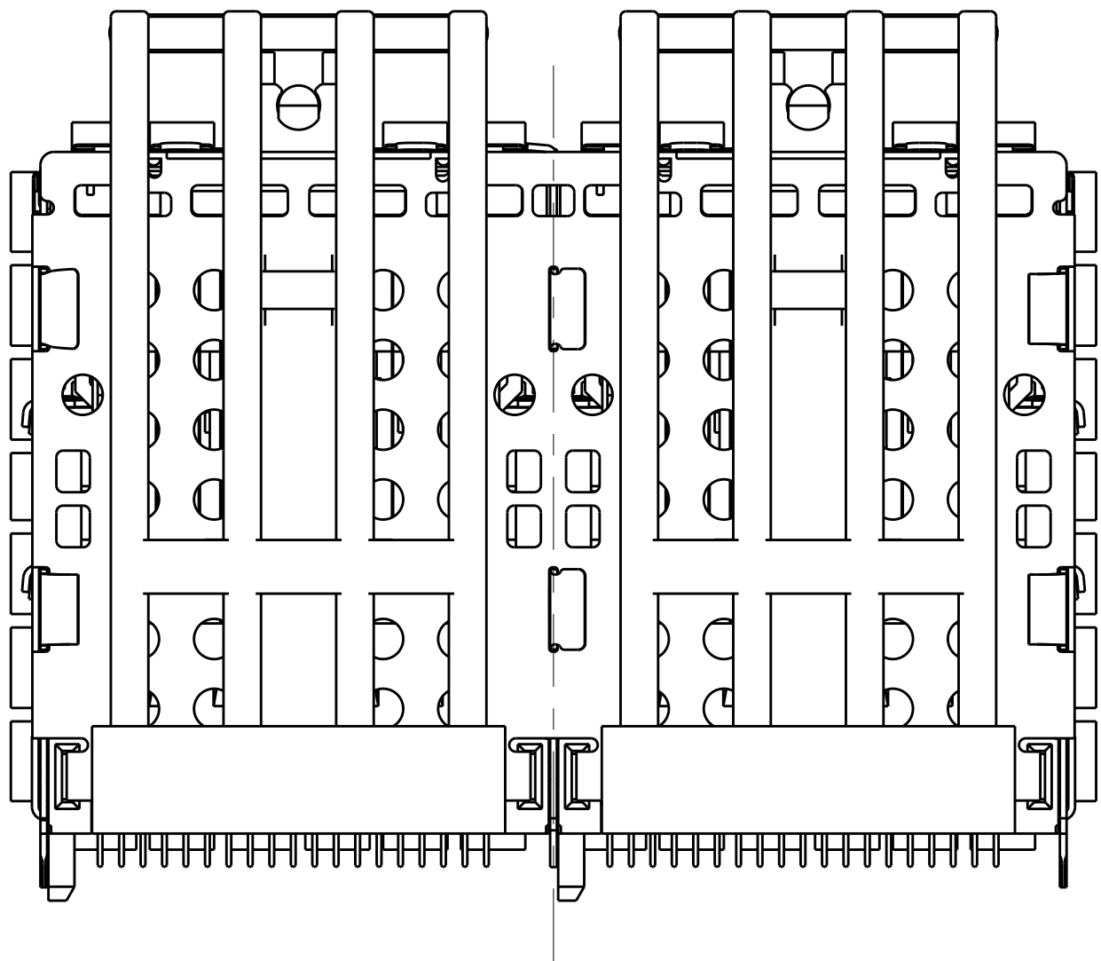
VIEW Y-Y
