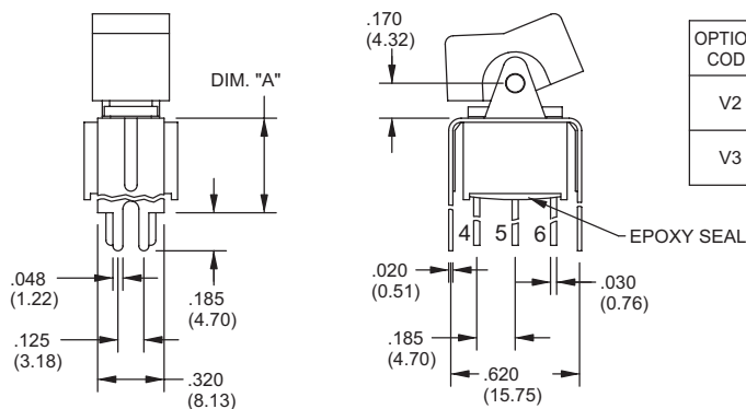
DPDT
