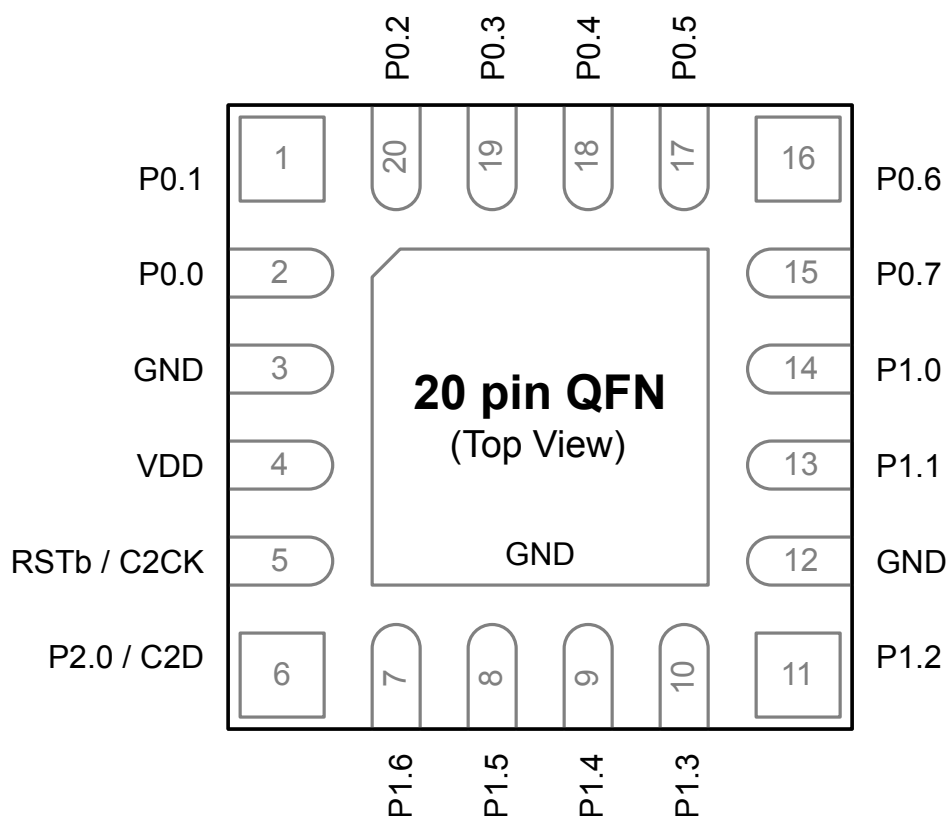
Figure 6.3. EFM8BB52-QFN20 Pinout
