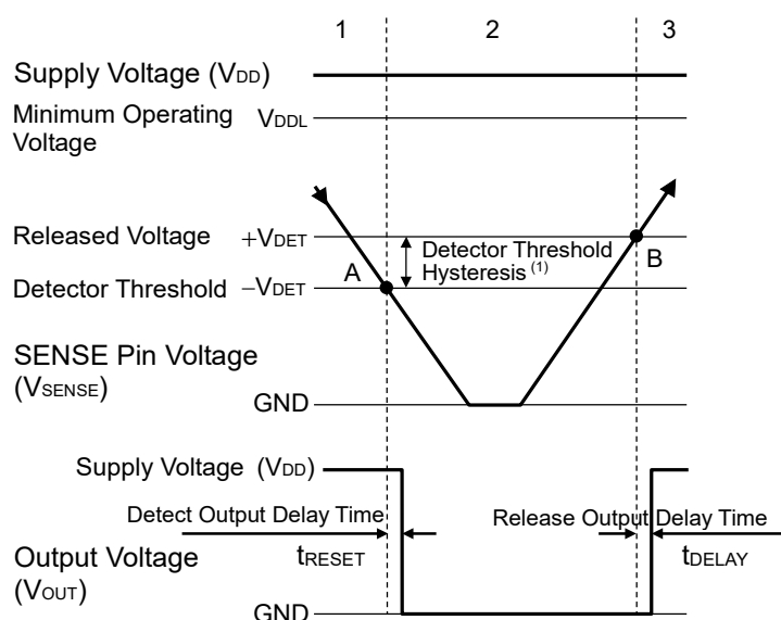
Operation Diagram
