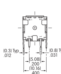
Sculptured Snap-on Cap • Straight PC
