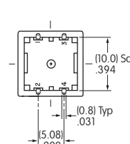
Flat Snap-on Cap • Straight PC
