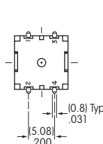
Flat Blue Button • Right Angle PC
