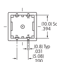
Sculptured Snap-on Cap • Straight PC
