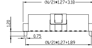
WITH POST STYLE 3, P/N: 20021321-3XXXXXL
