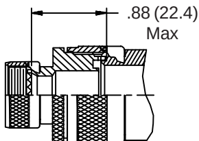
STYLE 2 (45° & 90° See Note 1)
