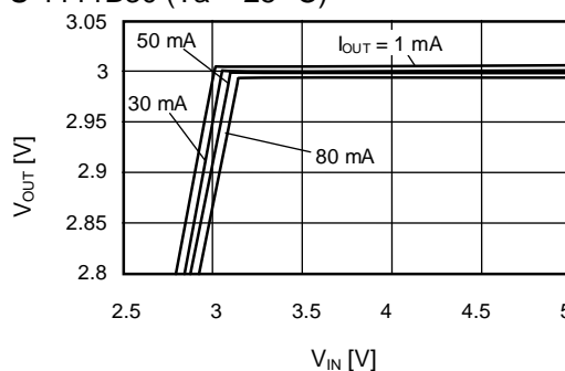
S-1111B30 ( T_a = 25^\circ\text{C} )
