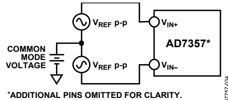
Figure 20. Differential Input Definition
