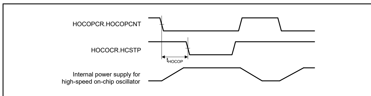
Figure 2.10 High-Speed On-Chip Oscillator Power Supply Control Timing
