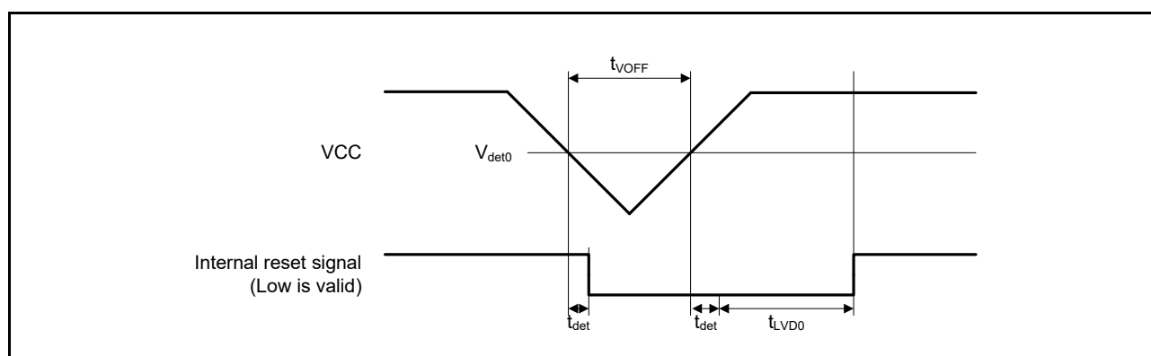
Figure 2.68 Voltage Detection Circuit Timing ( V_{det0} )
