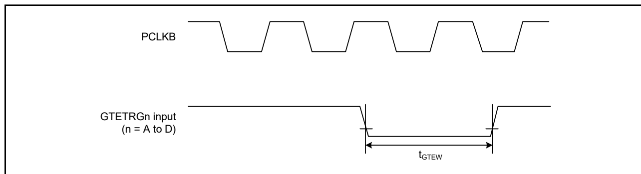
Figure 2.42 GPTW External Trigger Input Timing
