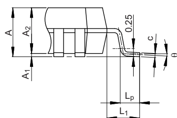
Detail F
