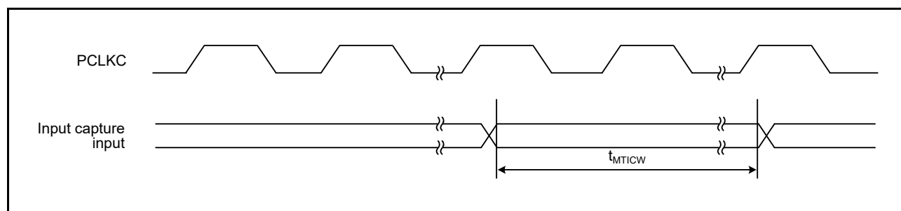
Figure 2.25 MTU Input Capture Input Timing
