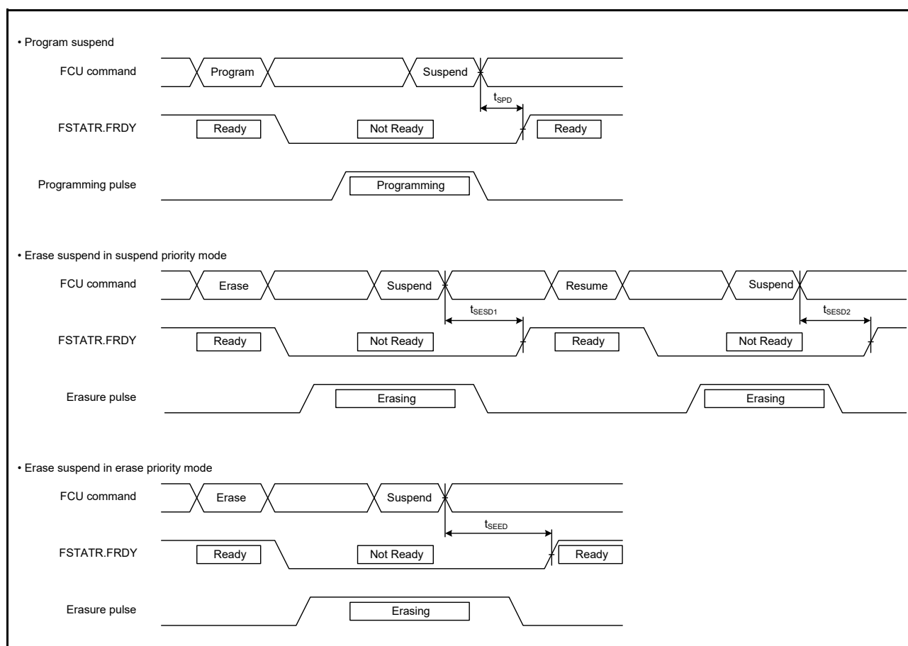
Figure 2.72 Flash Memory Program/Erase Suspend Timing
