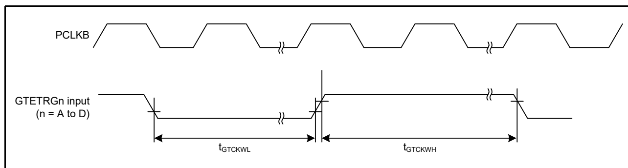
Figure 2.43 GPTW Clock Input Timing
