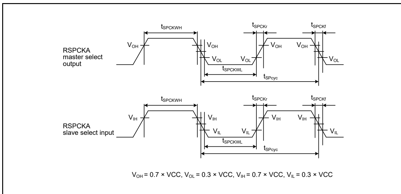
Figure 2.53 RSPI Clock Timing
