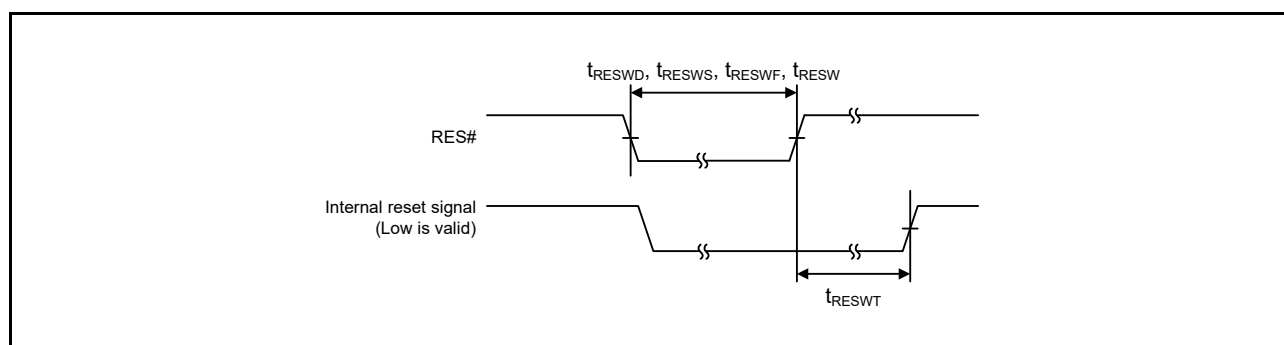
Figure 2.3 Reset Input Timing
