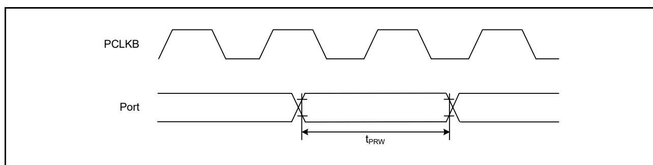
Figure 2.23 I/O Port Input Timing
