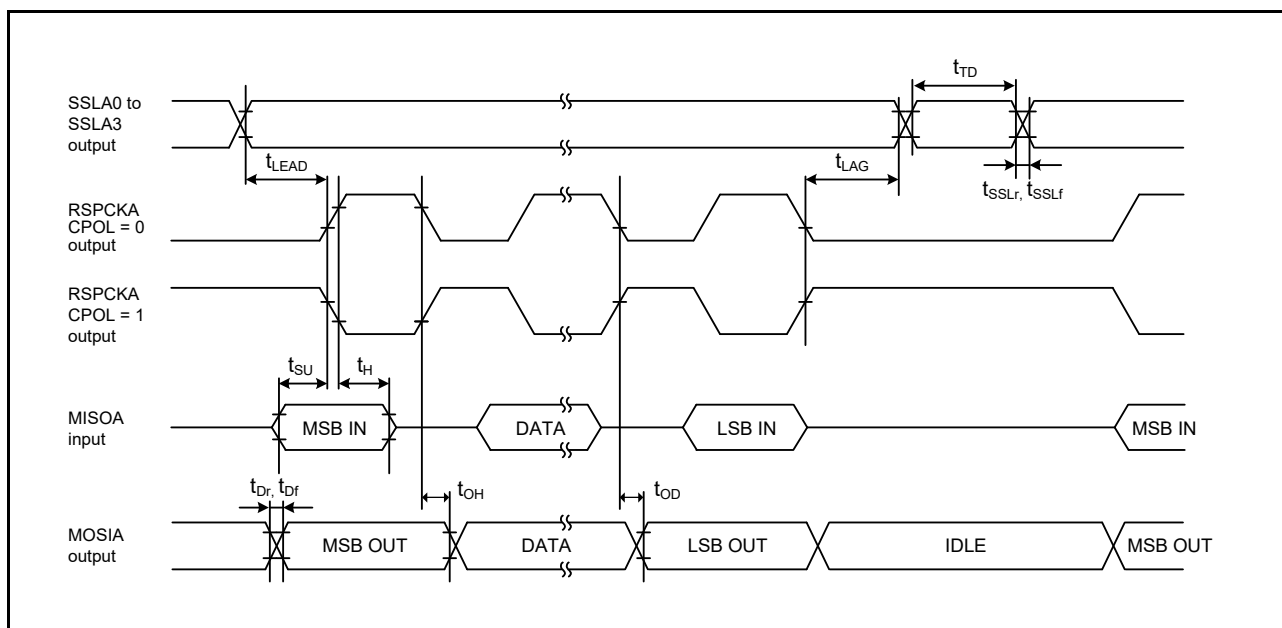
Figure 2.54 RSPI Timing (Master, CPHA = 0) (Bit Rate: PCLKA Division Ratio Set to a Value Other Than 1/2)
