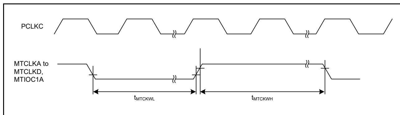
Figure 2.26 MTU Clock Input Timing
