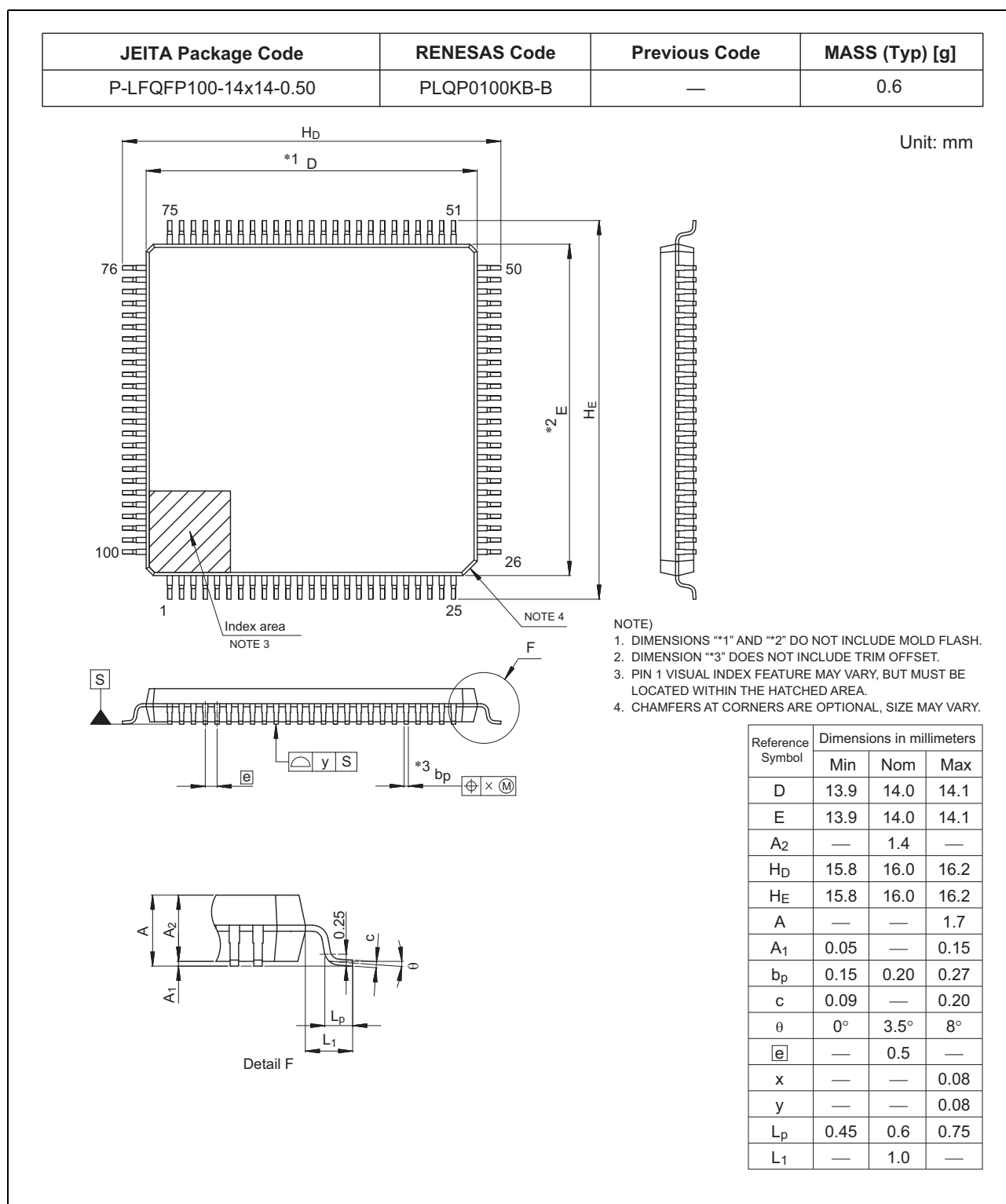
Figure C 100-Pin LFQFP (PLQP0100KB-B)
