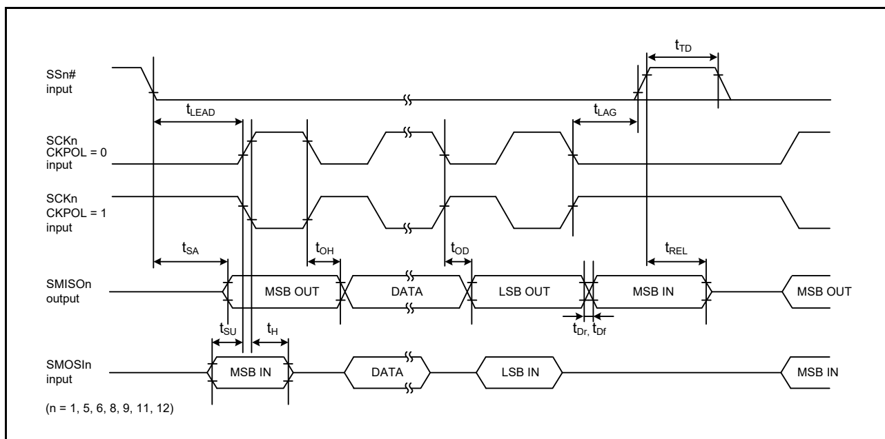
Figure 2.51 Simple SPI Timing (Slave, CKPH = 1)
