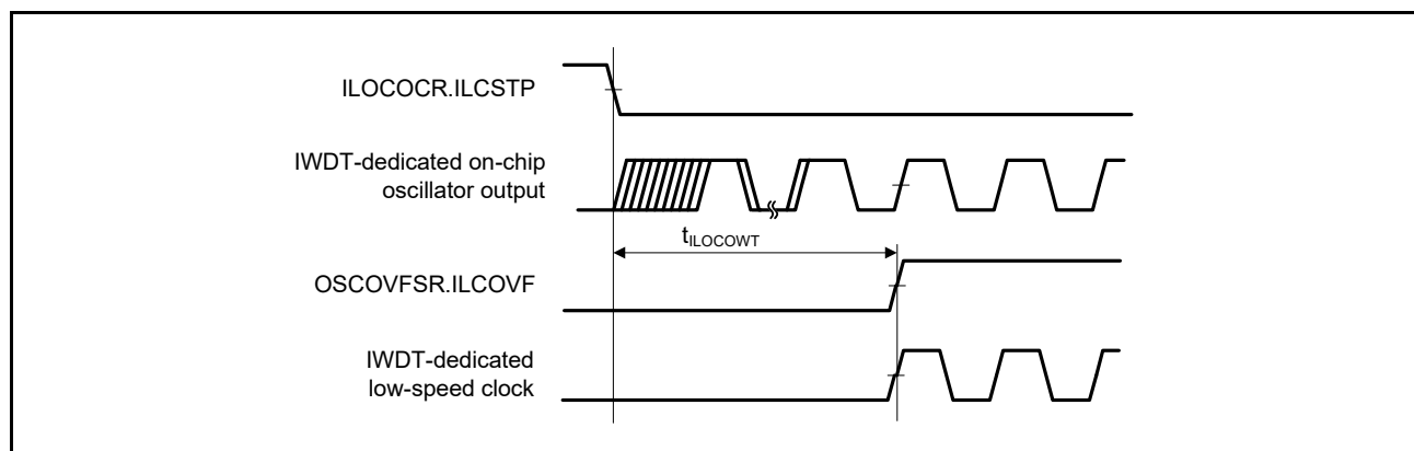
Figure 2.8 IWDT-dedicated Low-Speed Clock Oscillation Start Timing
