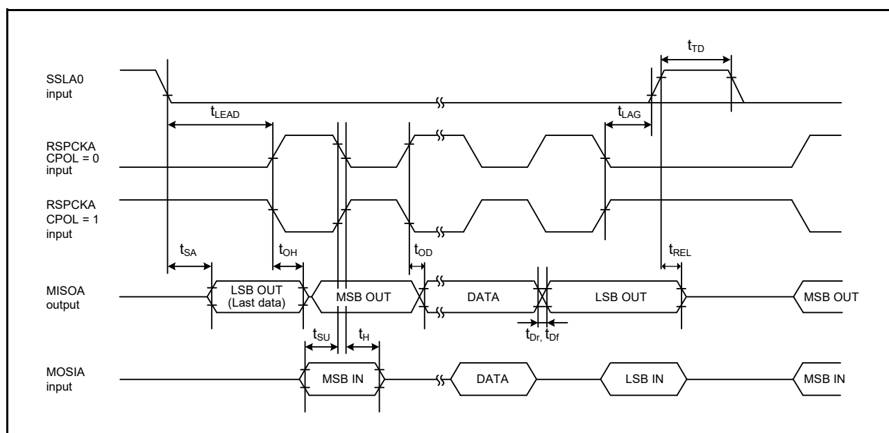
Figure 2.59 RSPI Timing (Slave, CPHA = 1)
