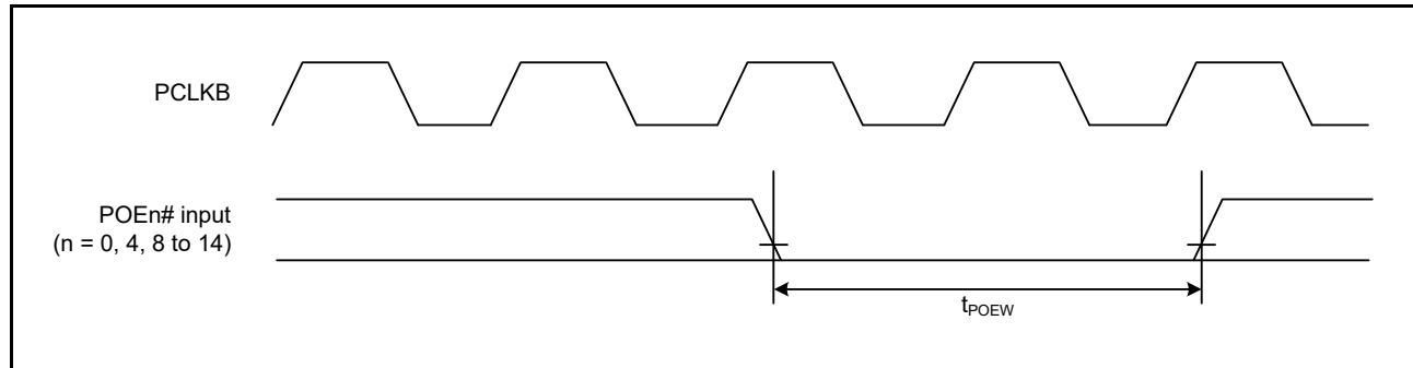
Figure 2.27 POE Input Timing
