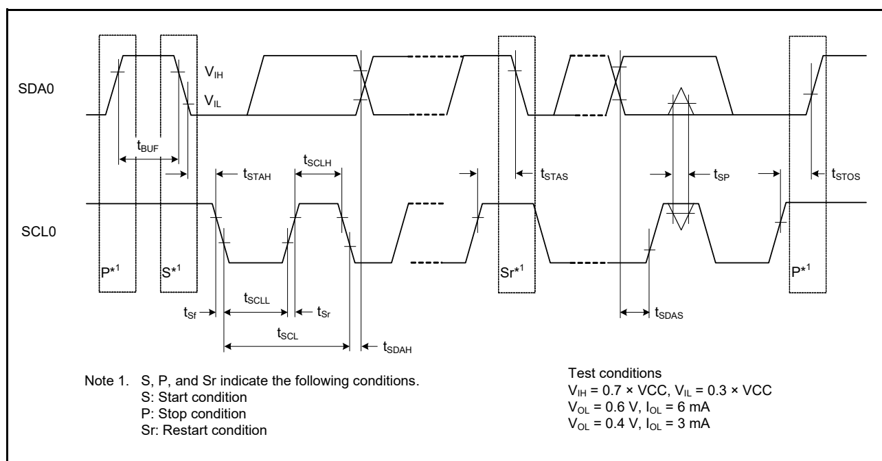
Figure 2.60 IIC Bus Interface Input/Output Timing
