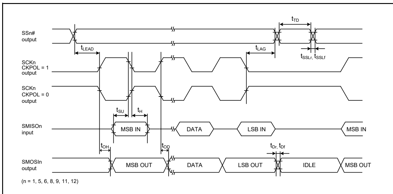
Figure 2.50 Simple SPI Timing (Master, CKPH = 0)
