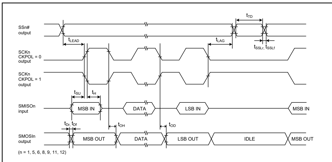
Figure 2.49 Simple SPI Timing (Master, CKPH = 1)
