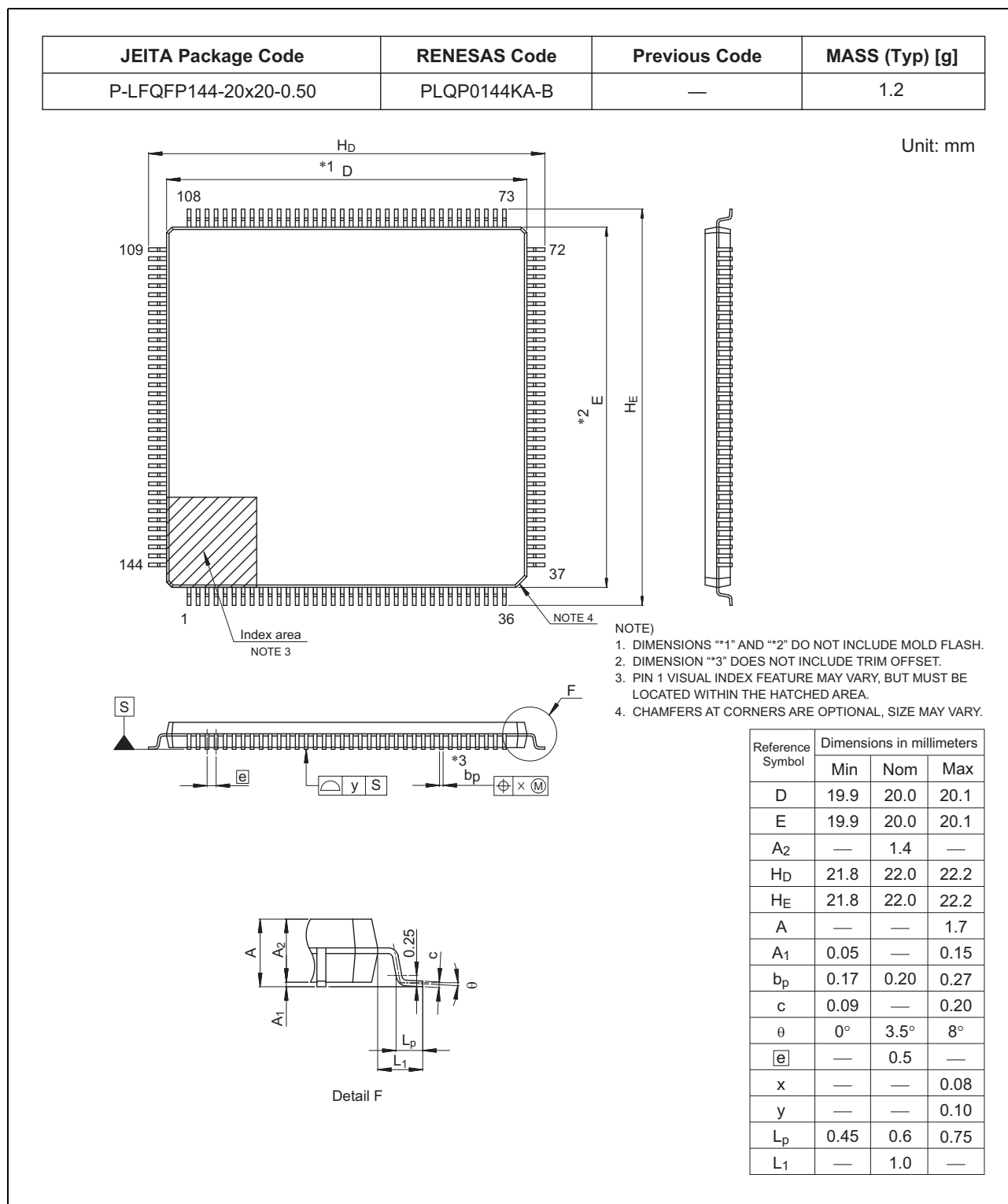
Figure A 144-Pin LFQFP (PLQP0144KA-B)
