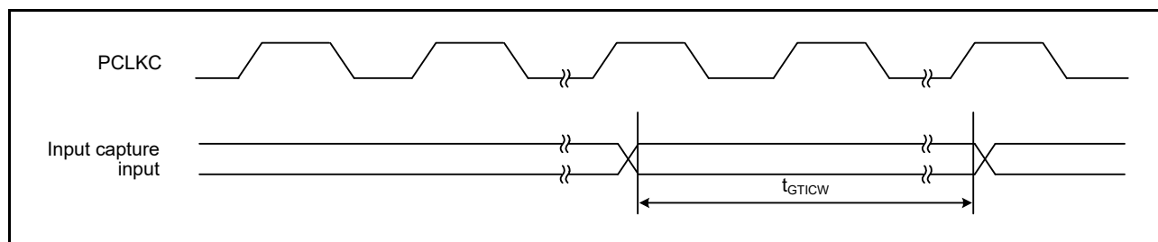
Figure 2.41 GPTW Input Capture Input Timing
