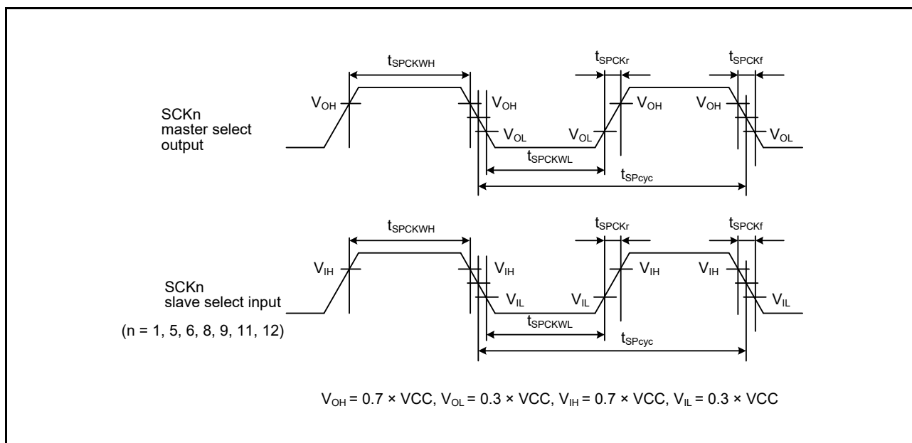
Figure 2.48 Simple SPI Clock Timing
