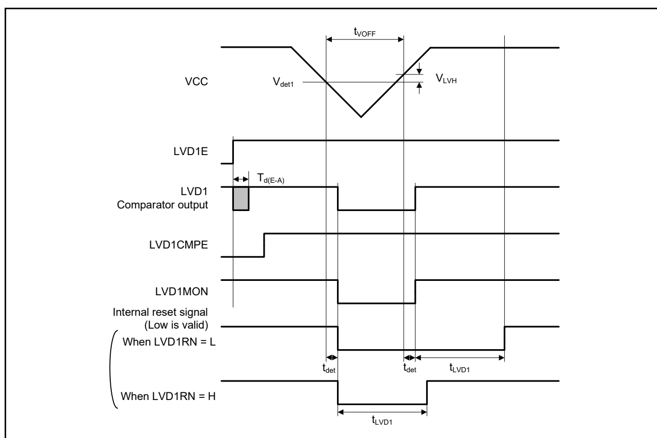
Figure 2.69 Voltage Detection Circuit Timing ( V_{det1} )
