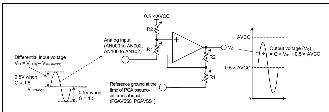
Figure 2.65 Input and Output Signal Levels with the PGA's Pseudo-Differential Setting
