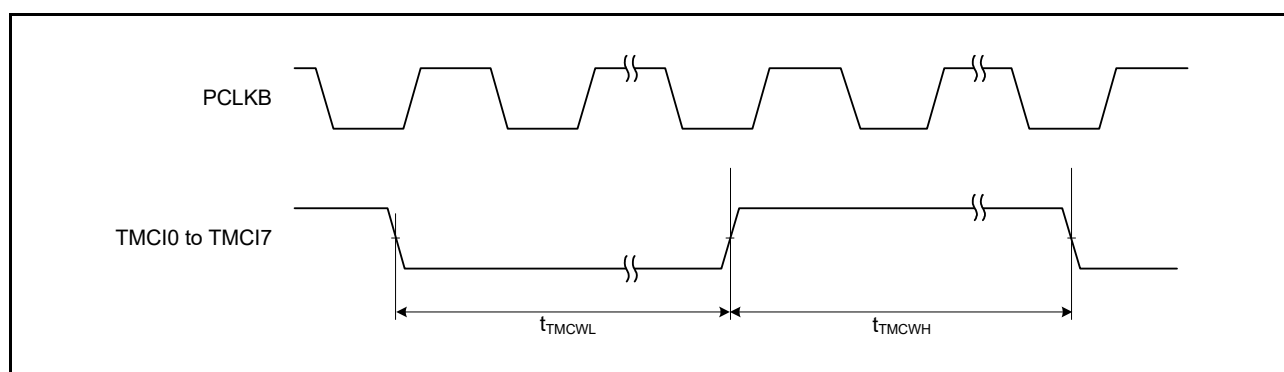
Figure 2.24 TMR Clock Input Timing
