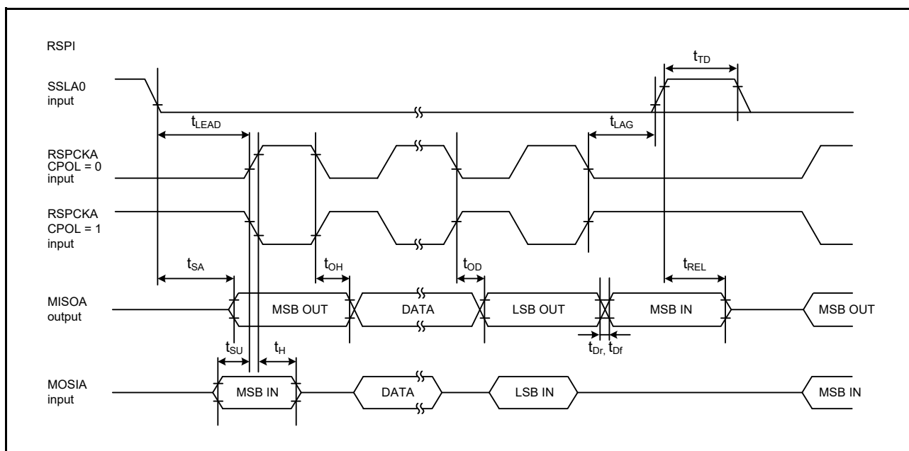
Figure 2.58 RSPI Timing (Slave, CPHA = 0)
