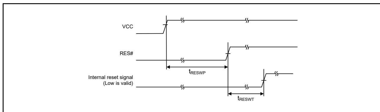
Figure 2.2 Reset Input Timing at Power-On
