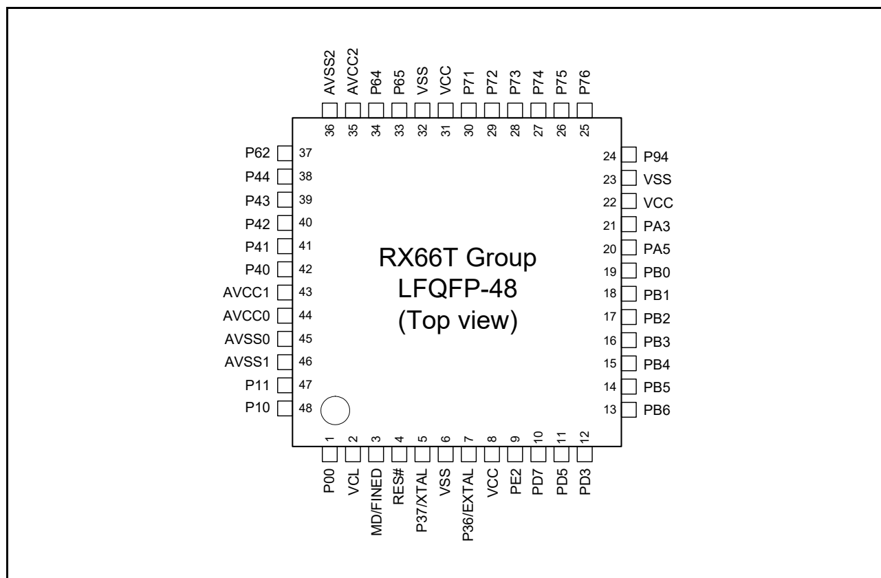
Figure 1.10 Pin Assignment (48-pin LFQFP) without PGA pseudo-differential input and without USB pin
