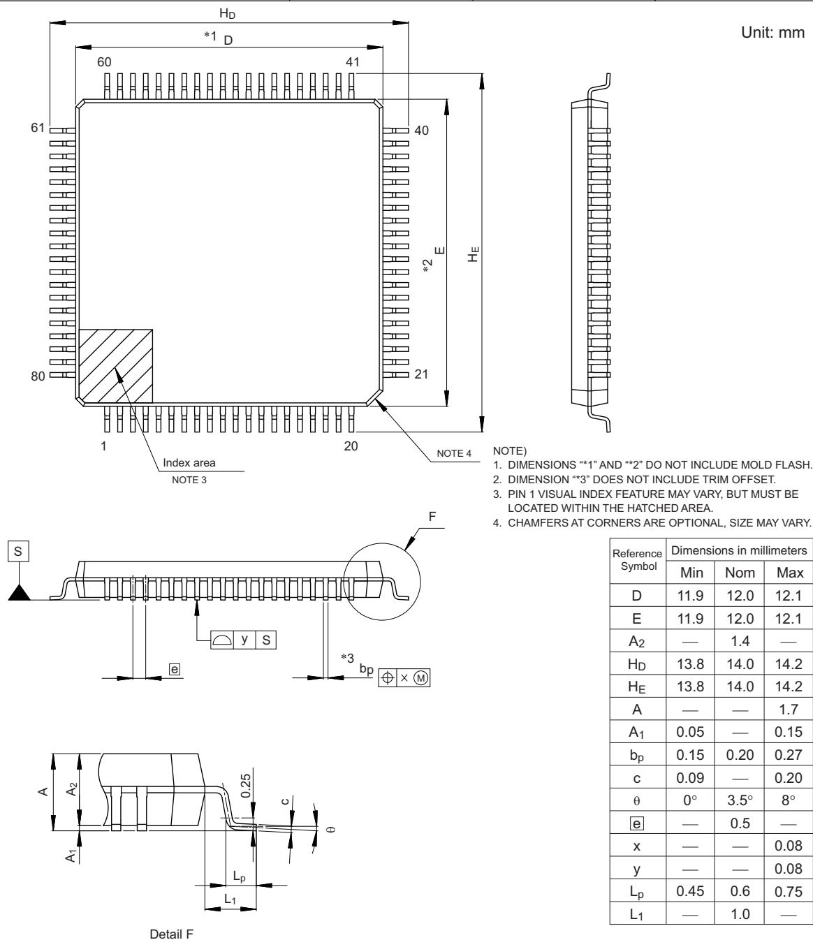
Figure E 80-Pin LFQFP (PLQP0080KB-B)
