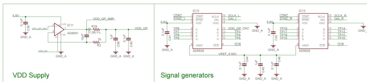
Figure 40: Signal Generator
