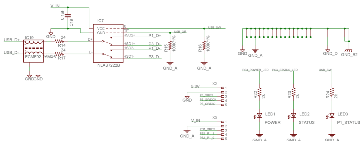
Figure 43: USB Protection
