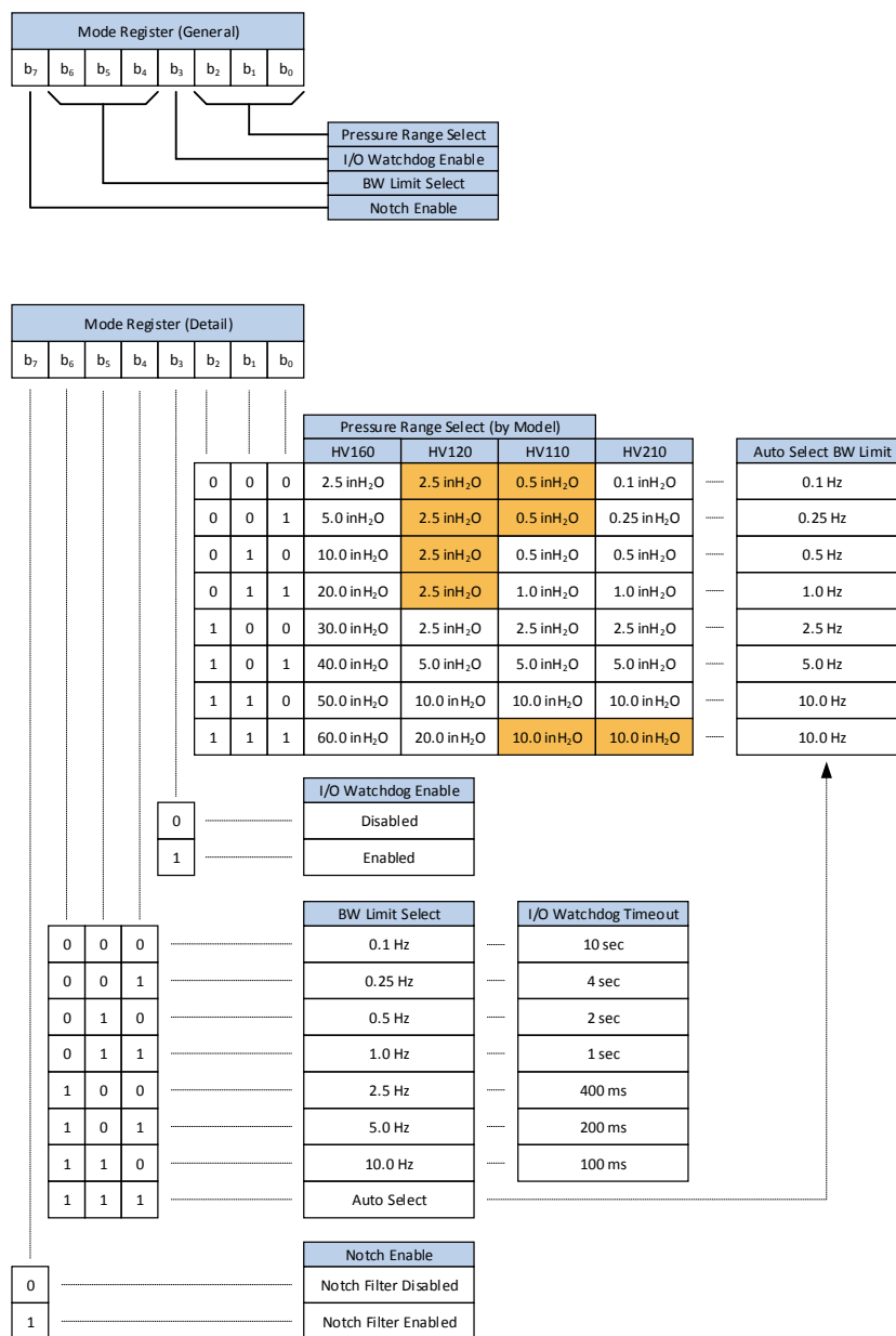
Mode Control Register Detail
