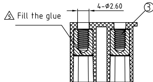
SECTION Q-Q
