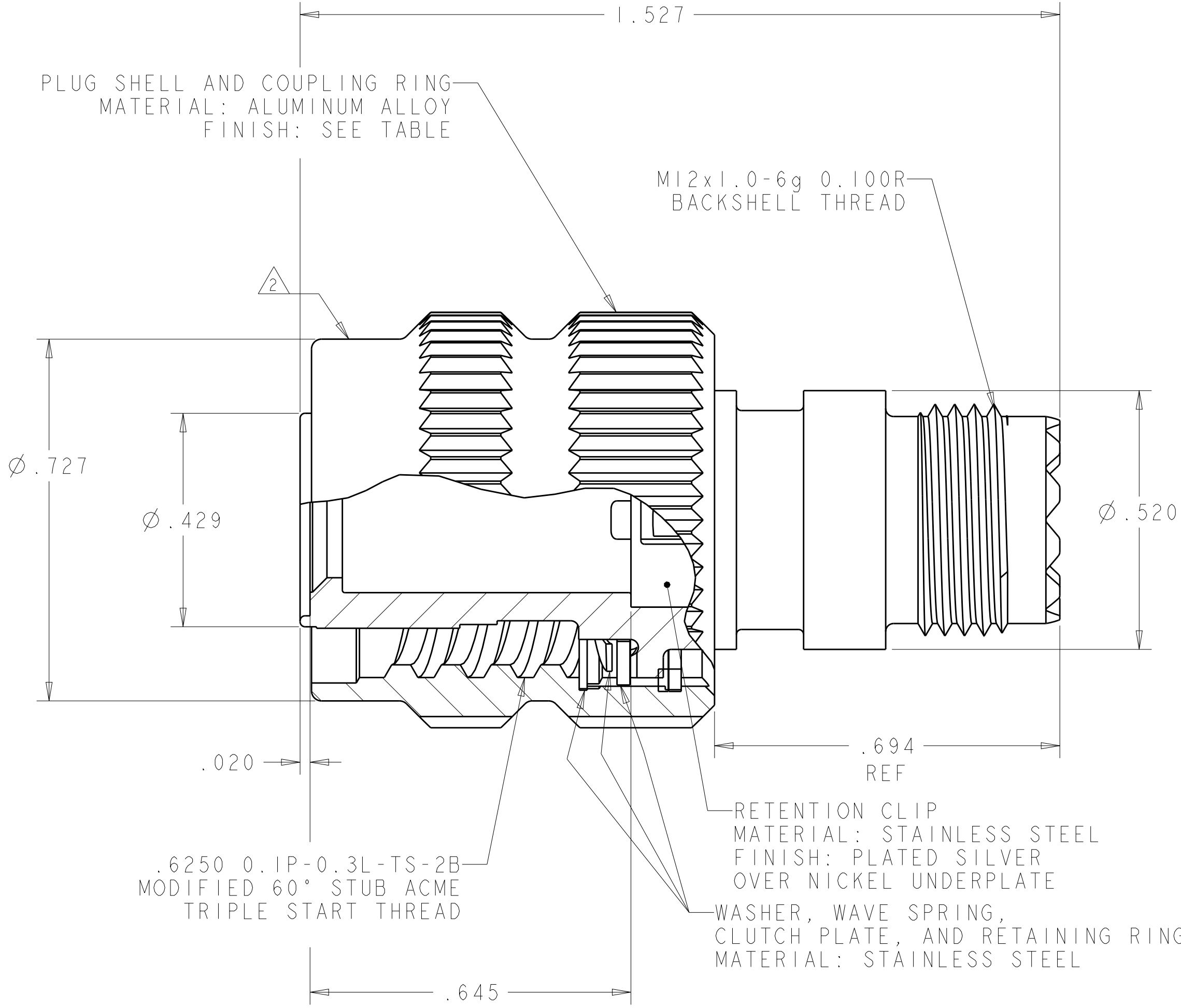
SECTION X-X
