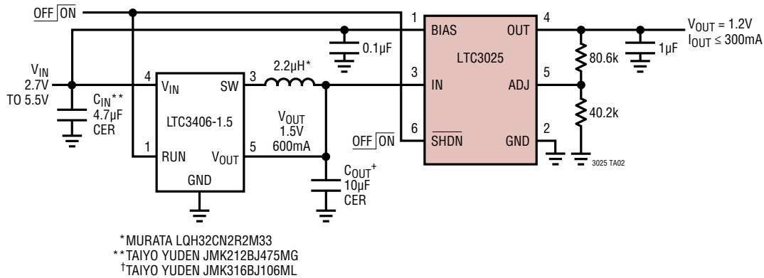
High Efficiency 1.5V Step-Down Converter with Efficient 1.2V VLDO Output
