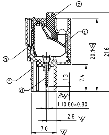
SECTION P-P
