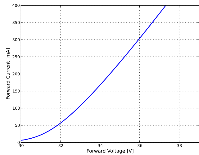
L2C5-xxHG1202E0900
