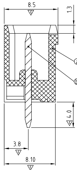
SECTION Q-Q
