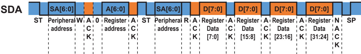
Figure 31: EEPROM Read – I²C Mode Blue represents data sent by the controller and orange is the data sent by the peripheral.
