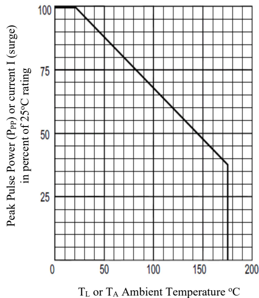
FIG. 4 Derating Curve
