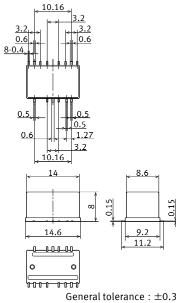
External dimensions
