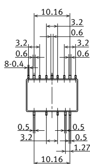
External dimensions
