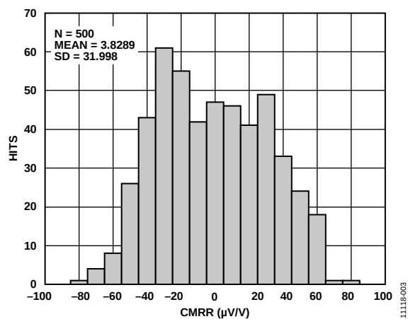
Figure 6. CMRR Distribution
