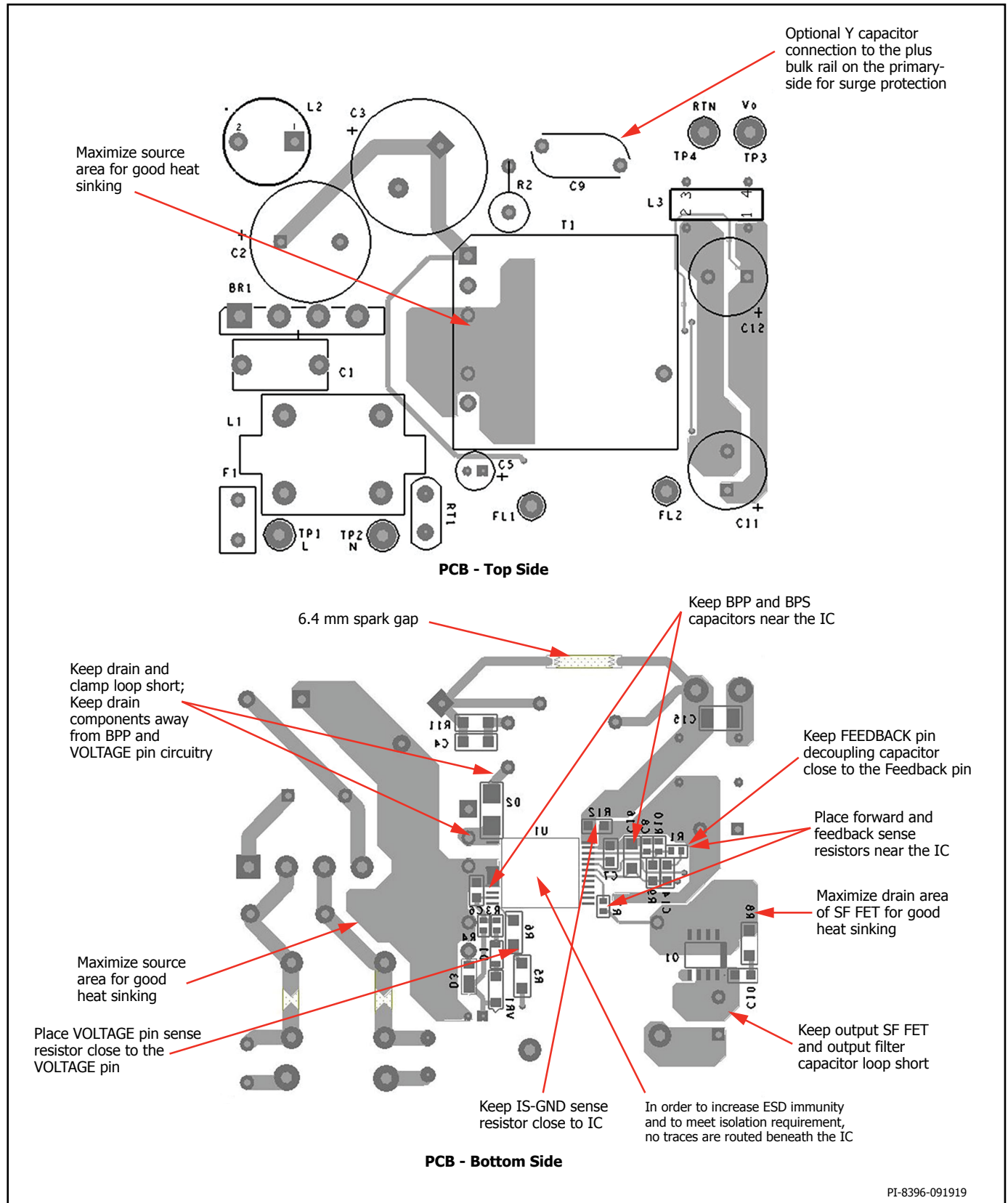
Figure 18. PCB.
