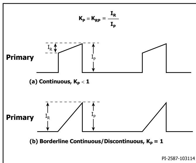
Figure 19. Continuous Conduction Mode Current Waveform, K_P < 1 .
