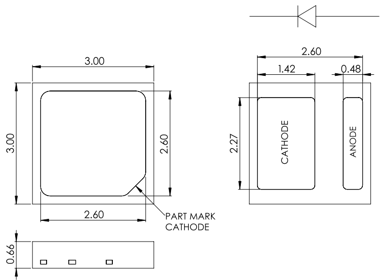
Figure 10. Mechanical dimensions for LUXEON 3030 HE.
