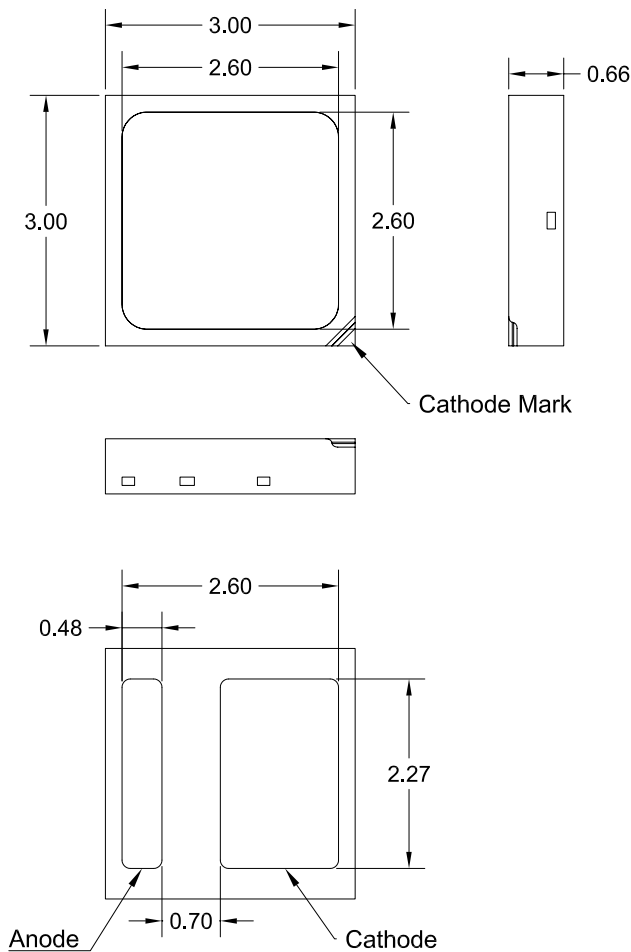
Figure 11. Mechanical dimensions for LUXEON 3030 HE Plus.
