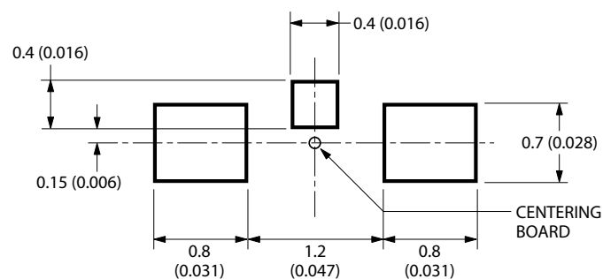
Figure 15: Recommended Soldering Pattern for HSMx-C120
