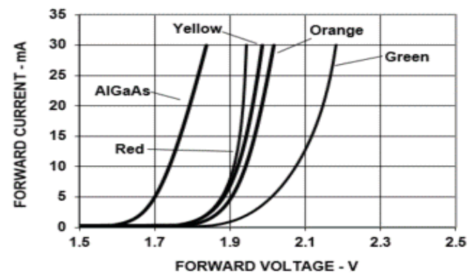
Figure 2: Forward Current vs. Forward Voltage
