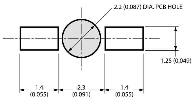
Figure 16: Recommended Soldering Pattern for HSMx-C265
