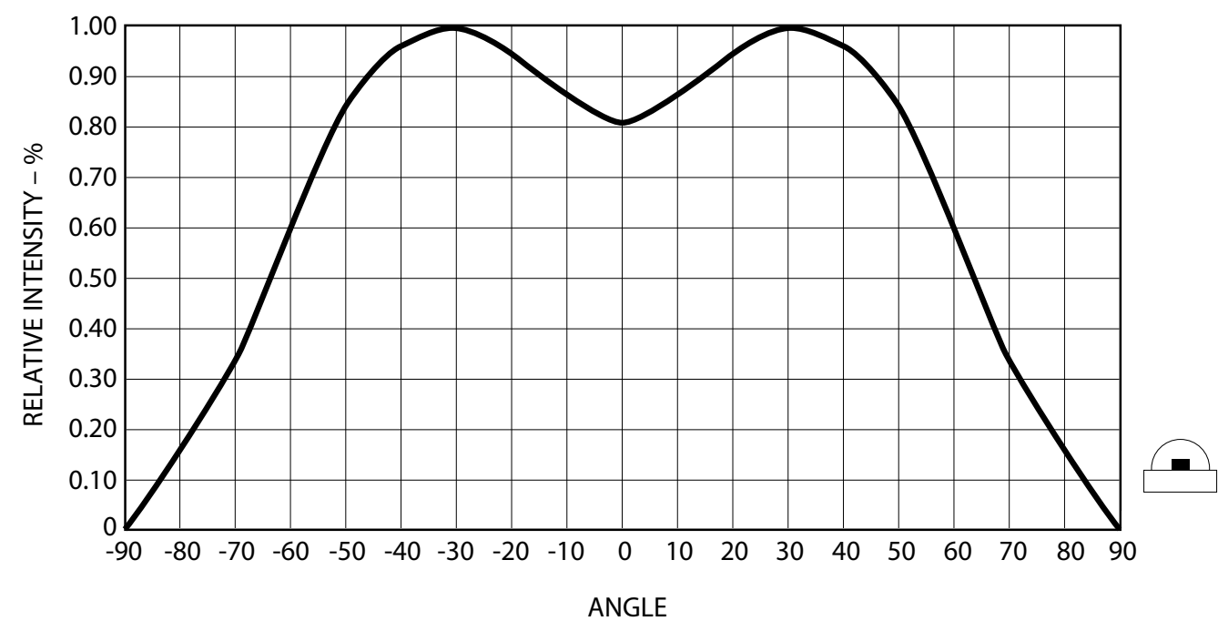
Figure 5: Relative Intensity vs. Angle for HSMx-C110
