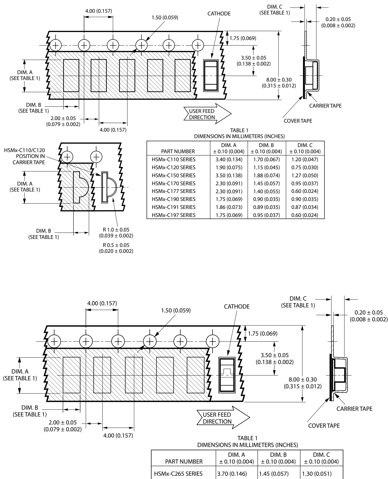
Figure 19: Tape Dimensions
