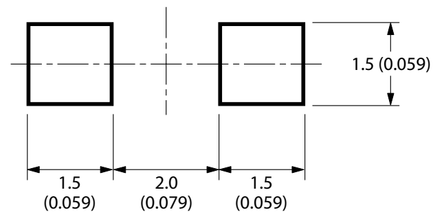
Figure 11: Recommended Soldering Pattern for HSMx-C150
