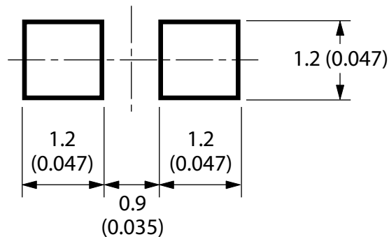
Figure 12: Recommended Soldering Pattern for HSMx-C170 and C177
