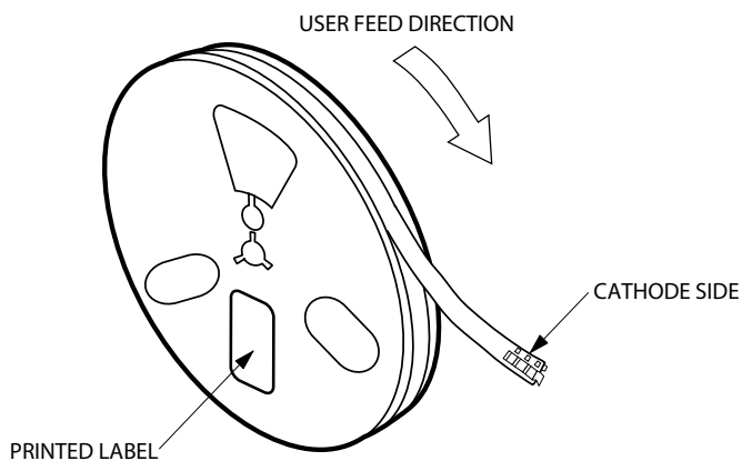
Figure 17: Reeling Orientation
