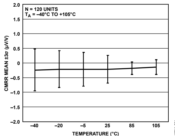
Figure 28. CMRR Mean vs. Temperature (Gain = 1 V/V)
