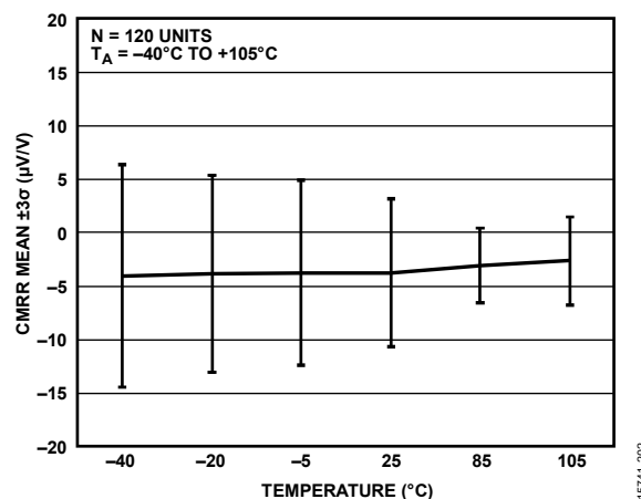
Figure 29. CMRR Mean vs. Temperature (Gain = 1/16 V/V)
