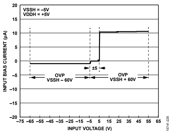
Figure 36. Input Overvoltage Performance, V_{DDH}/V_{SSH} = \pm 5\text{ V}
