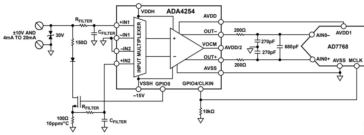
Figure 103. Voltage/Current Input Application
