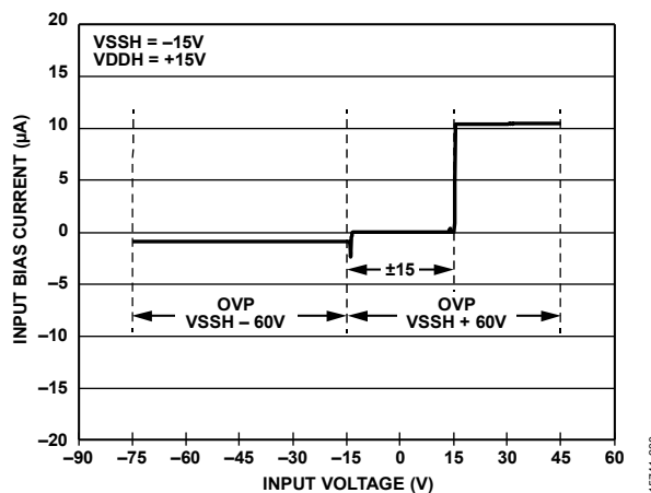
Figure 33. Input Overvoltage Performance, V_{DDH}/V_{SSH} = \pm 15\text{ V}
