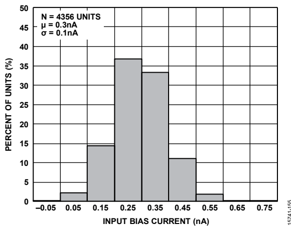
Figure 27. Input Bias Current Distribution
