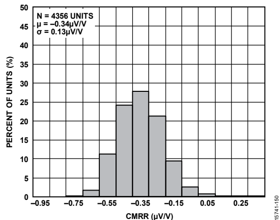
Figure 25. CMRR Distribution (Gain = 1 V/V)
