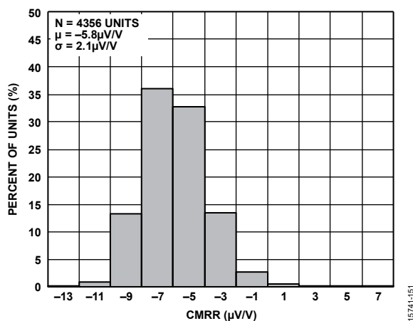
Figure 26. CMRR Distribution (Gain = 1/16 V/V)
