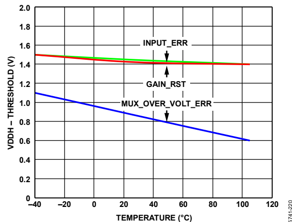
Figure 78. Error Flag Positive Trip Voltage ( V_{DDH} - Threshold) vs. Temperature
