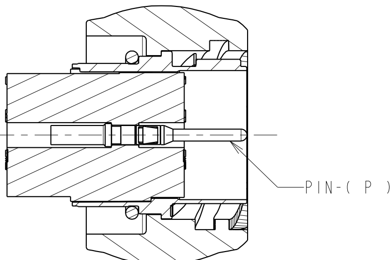
MALE CONNECTOR (Detail 1)
