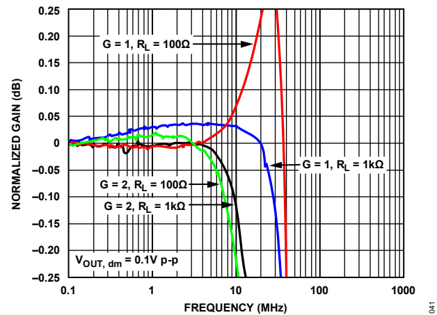
Figure 58. 0.1 dB Flatness Small Signal Frequency Response for Various Gains and Loads
