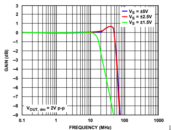
Figure 8. Large Signal Frequency Response for Various Supplies
