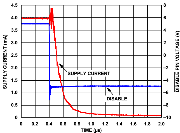
Figure 35. \overline{\text{DISABLE}} Pin Turn-Off Time
