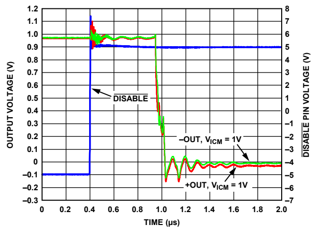
Figure 38. \overline{\text{DISABLE}} Pin Turn-On Time
