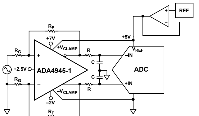
Figure 113. ADA4945-1 Output Voltage Clamp Usage
