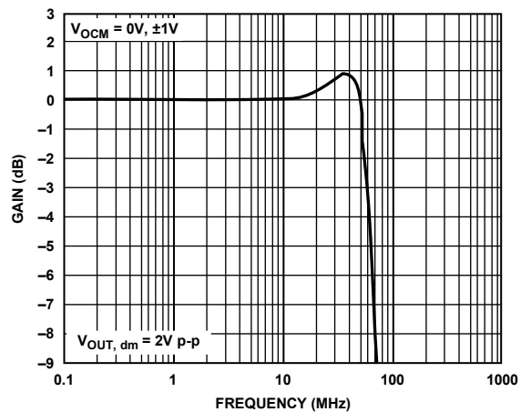
Figure 11. Large Signal Frequency Response at Various V_{OCM} Levels
