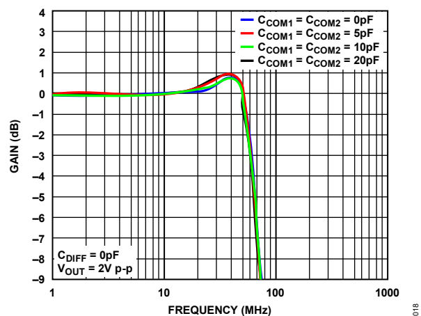
Figure 15. Large Signal Frequency Response for Various Capacitive Loads
