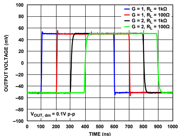
Figure 39. Small Signal Transient Response for Various Gains and Loads
