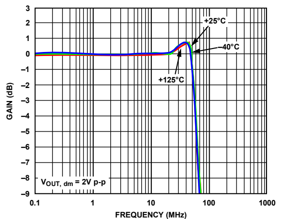
Figure 9. Large Signal Frequency Response for Various Temperatures
