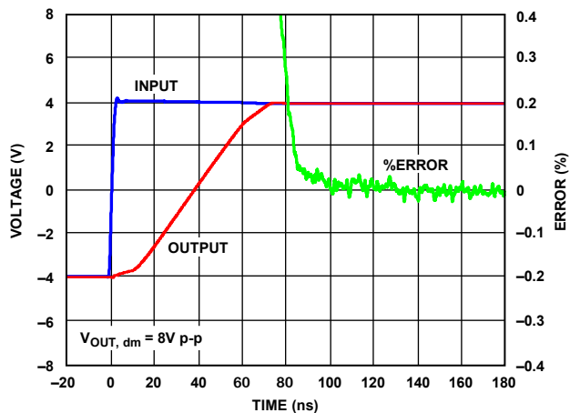
Figure 81. 0.1% Settling Time
