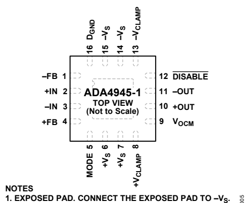
Figure 3. Pin Configuration
