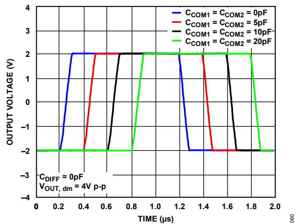
Figure 91. Large Signal Transient Response for Various Capacitive Loads, V_S = 3V
