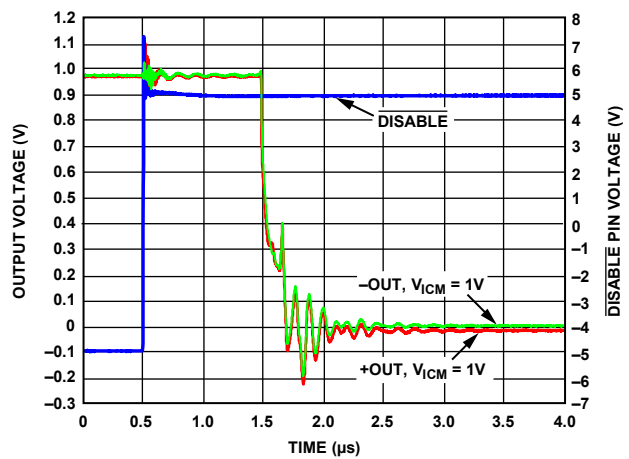
Figure 83. \overline{\text{DISABLE}} Pin Turn-On Time
