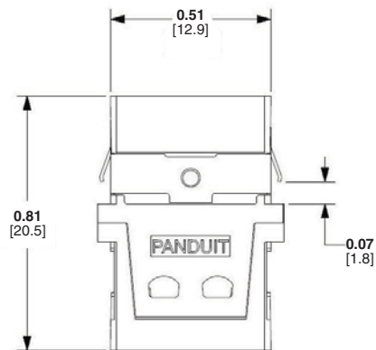
Top view of MPO adapter
