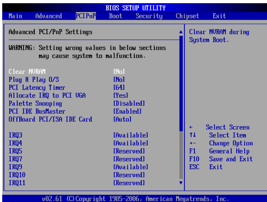
Figure 4.18: PCI/PnP Setup
