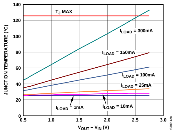
Figure 38. Junction Temperature vs. Power Dissipation, 500 mm 2 of PCB Copper, T_A = 25^\circ\text{C}
