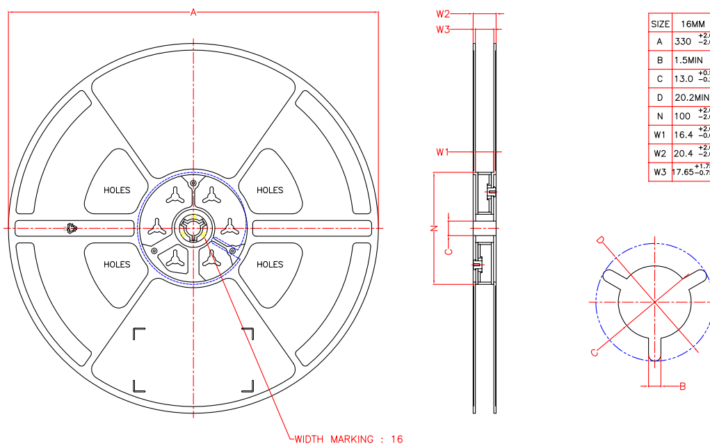
Figure 10.2. Reel Dimensions
