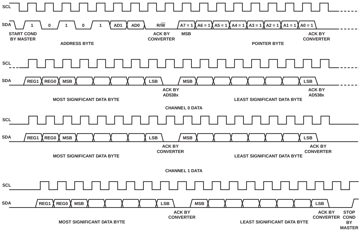
Figure 33. 2-Byte, I²C Write Operation
