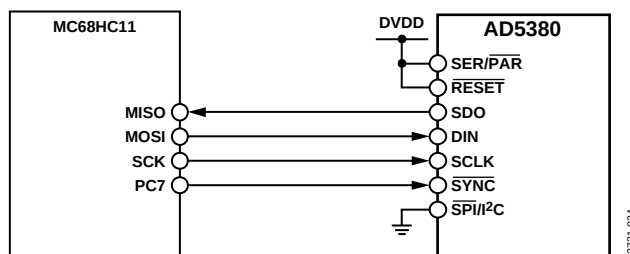
Figure 34. AD5380-to-MC68HC11 Interface
