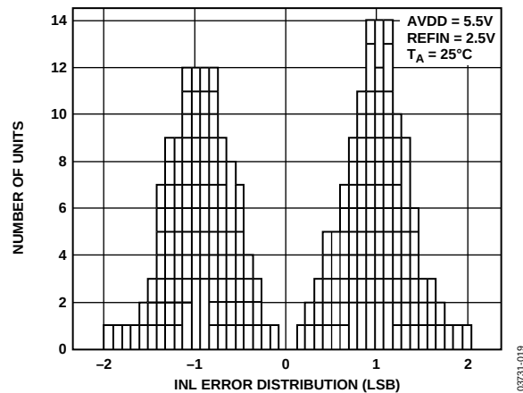
Figure 19. INL Distribution
