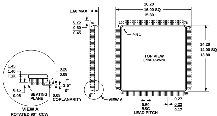
COMPLIANT TO JEDEC STANDARDS MS-026-BED Figure 50. 100-Lead Low Profile Quad Flat Package [LQFP] (ST-100-1) Dimensions shown in millimeters
