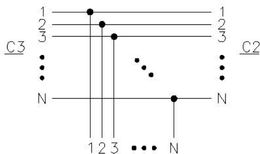
Connection Diagram
