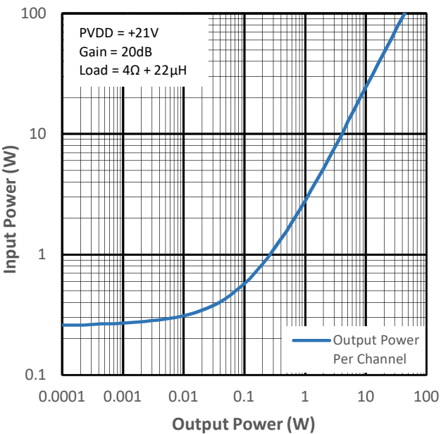
Figure 14-16 Input Power vs Output Power for PMP4
