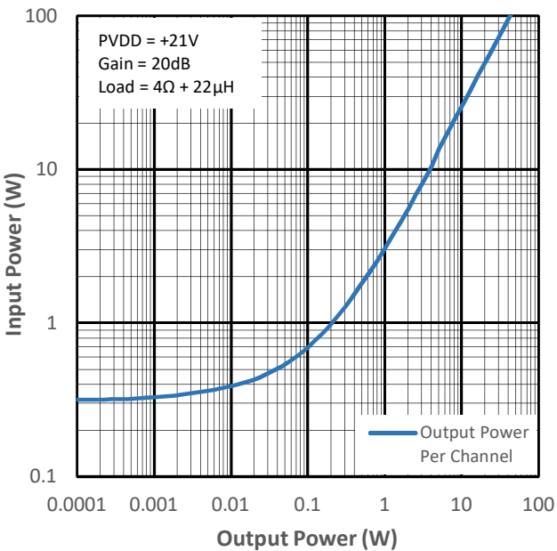
Figure 14-14 Input Power vs Output Power for PMP1
