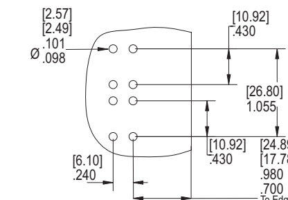
PCB Hole Layout for Double Powerpole
