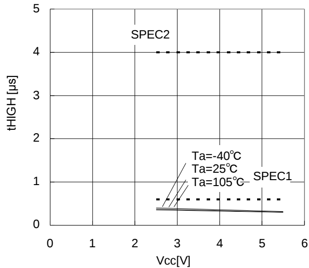
Figure 15. Data clock "H" time t_{HIGH}
