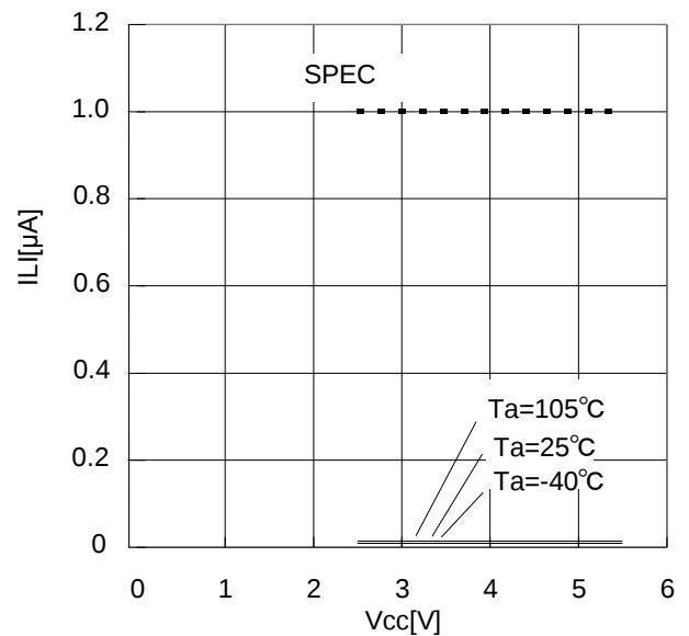
Figure 5. Input leak current I_{IL1} (SCL, WP)
