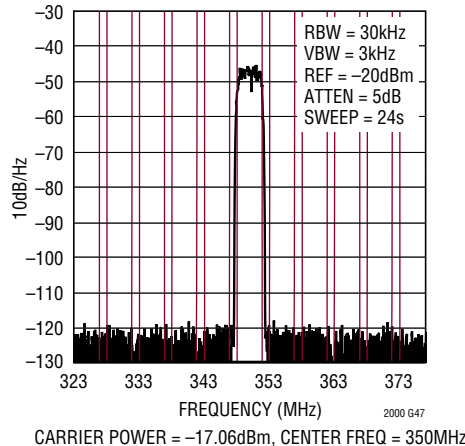
LTC2000-16 Single Carrier WCDMA ACLR at 350MHz, f_{DAC} = 2.5Gpsps
