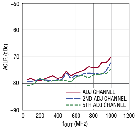
LTC2000-16 Single Carrier WCDMA ACLR vs f_{OUT} , f_{DAC} = 2.5Gpsps
