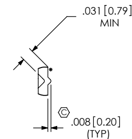
CRIMP DETAIL SCALE: 4:1 (TYP ALL CRIMPS)
