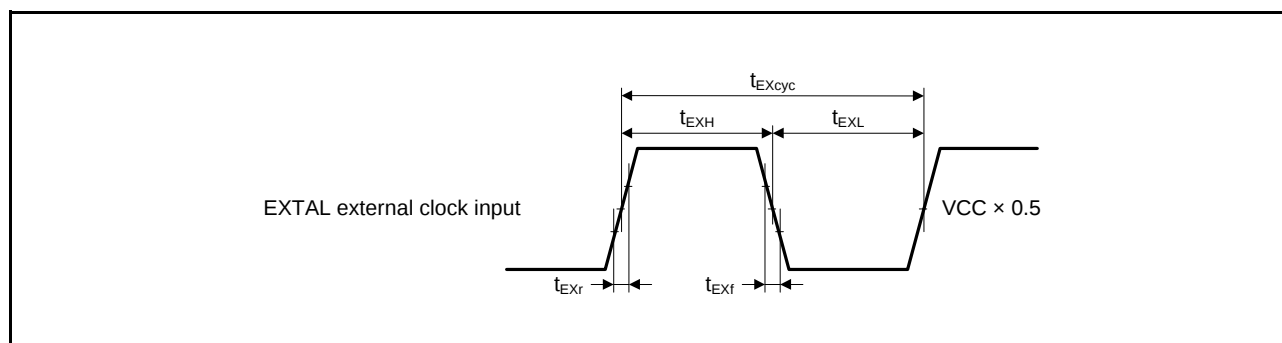
Figure 5.2 EXTERNAL External Clock Input Timing
