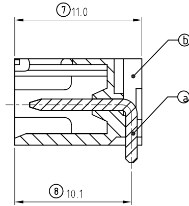
SECTION P-P
