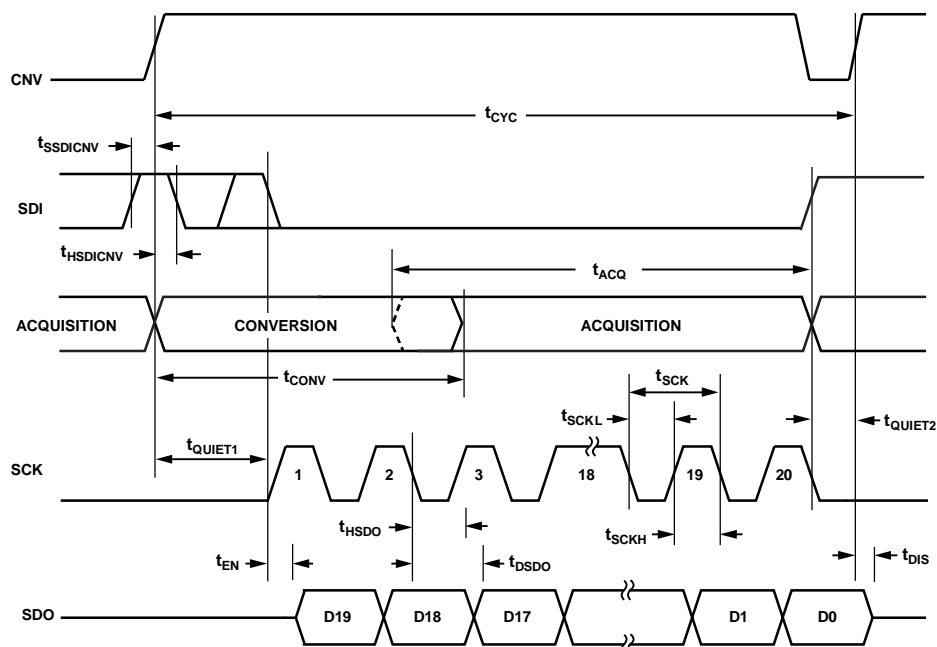
Figure 60. \overline{\text{CS}} Mode, 4-Wire Turbo Mode Timing Diagram (Status Bits Not Shown)
