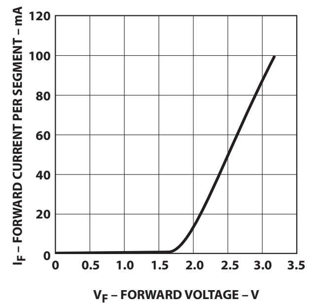
Figure 2: Forward Current vs. Forward Voltage
