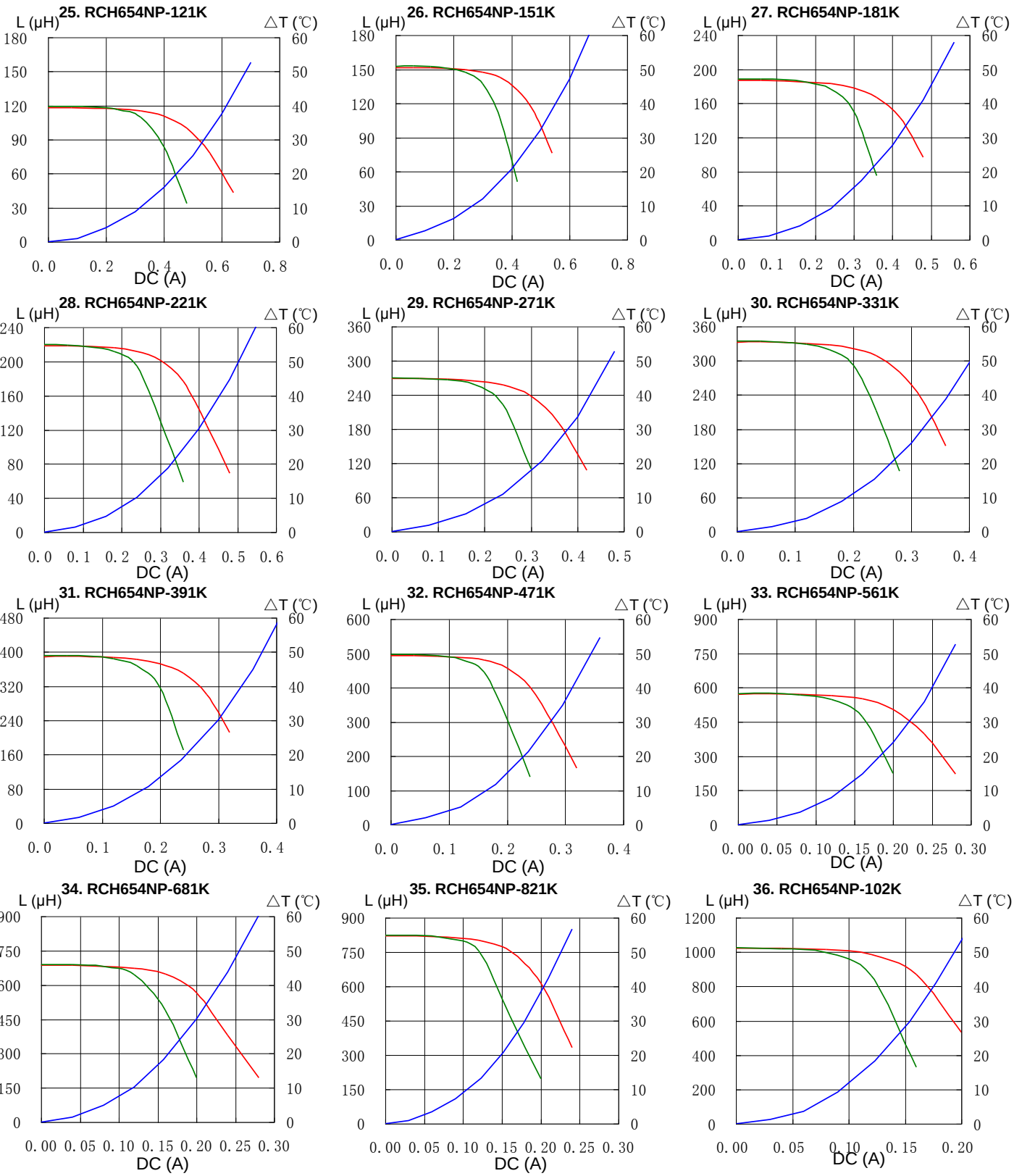
Saturation Current & Temperature Rise Graph
