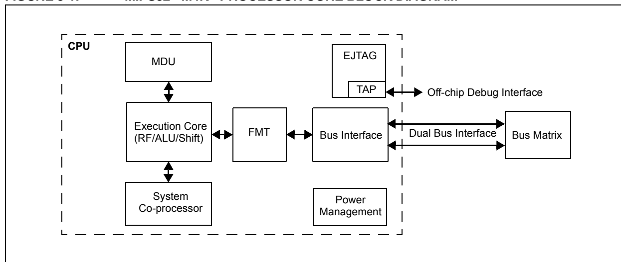
FIGURE 3-1: MIPS32® M4K® PROCESSOR CORE BLOCK DIAGRAM
