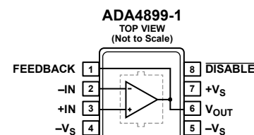
Figure 1. 8-Lead LFCSP (CP-8-13)
