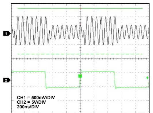
Figure 52. ADA4899-1 2:1 Mux Transient Response
