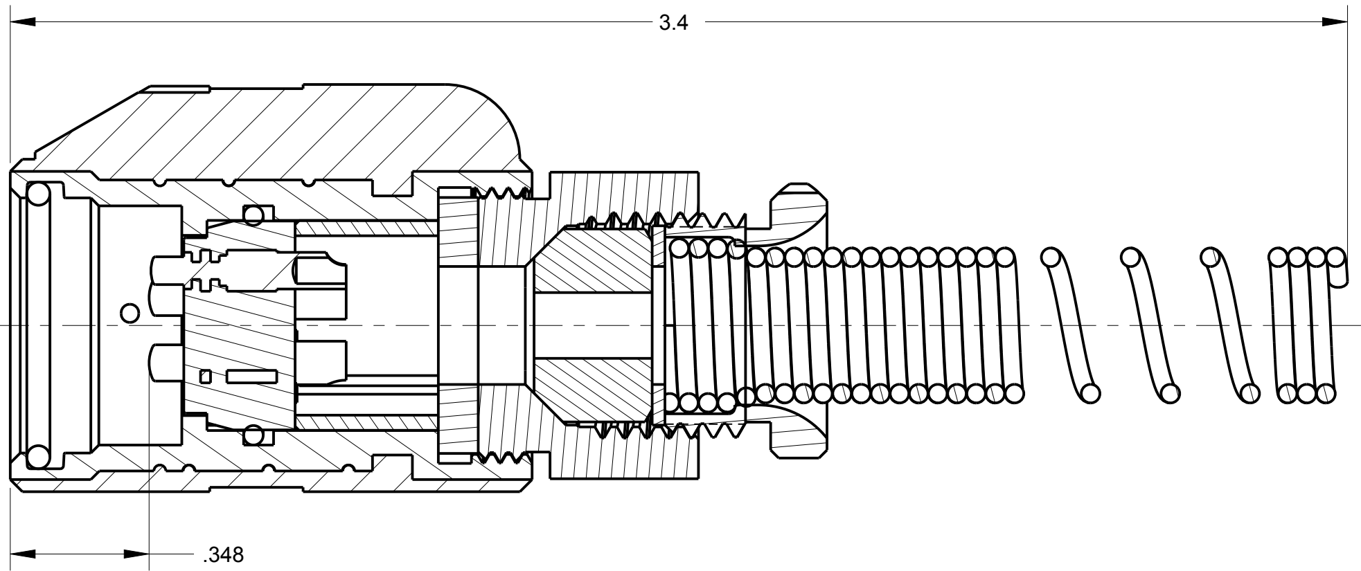
SECTION Z-Z
