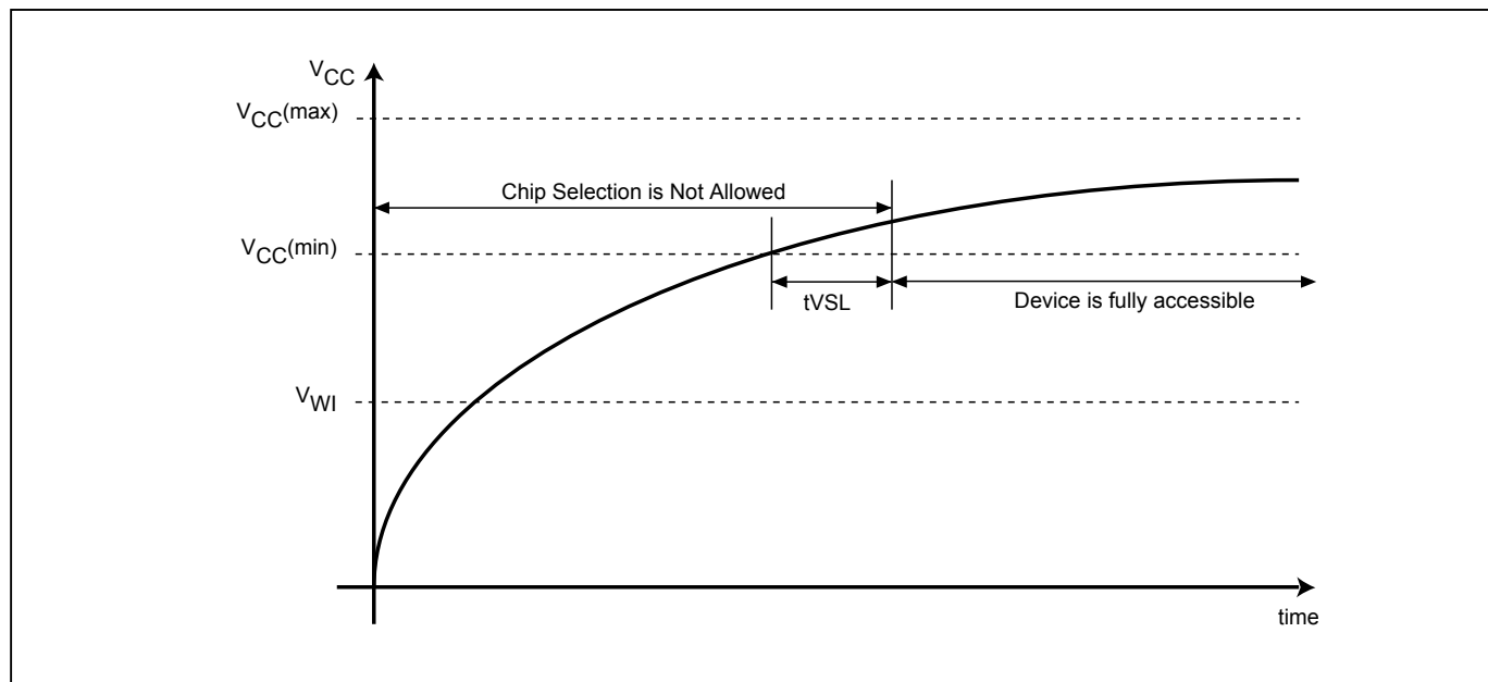
Figure 49. Power-up Timing
