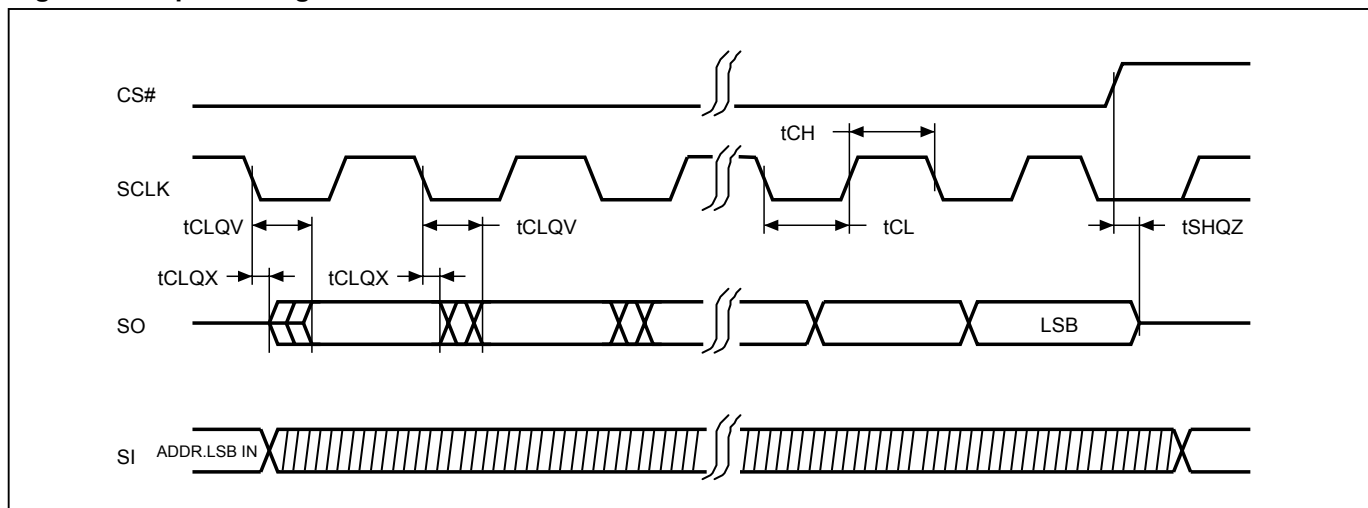
Figure 3. Output Timing
