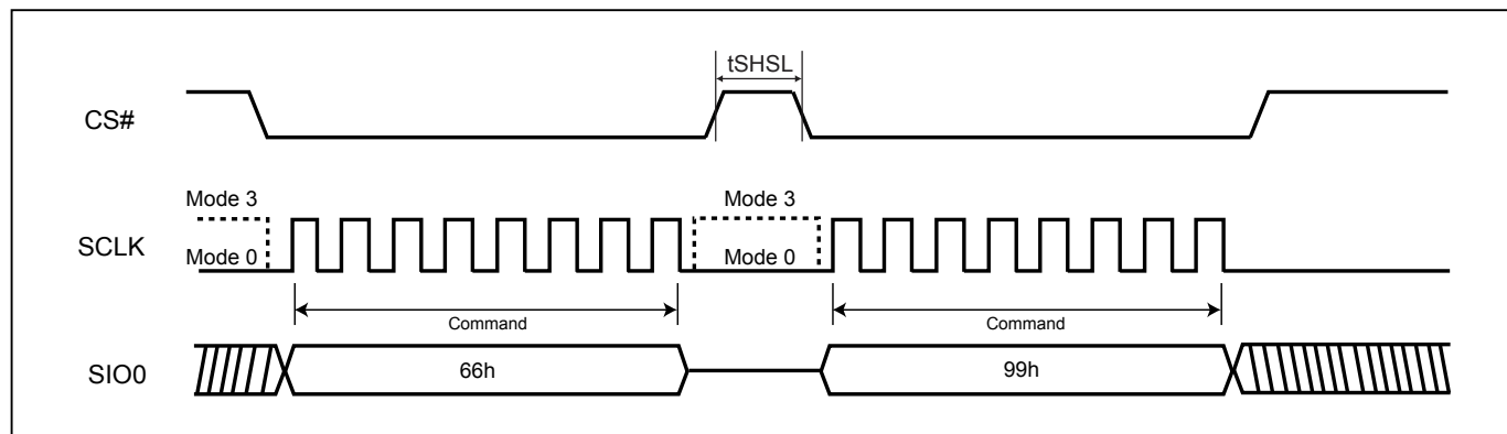
Figure 39. Reset Sequence
