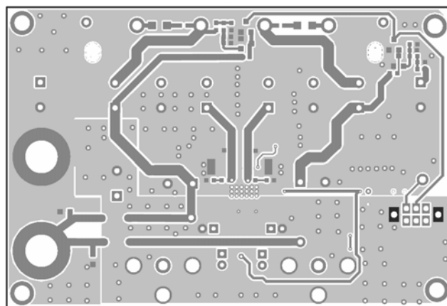
Figure 4—Bottom and Bottom Silk Layer
