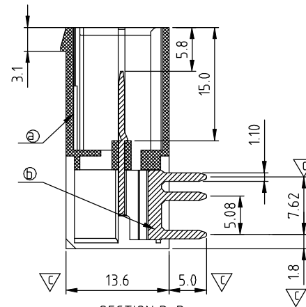
SECTION P-P
